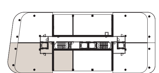
SOUTH TOWER
